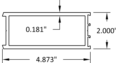
⑩⑦ MEETING STILE (ACTIVE)
