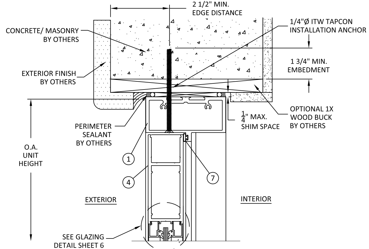
B 4 VERTICAL SECTION DOOR HEAD - CONCRETE/MASONRY THROUGH FRAME
