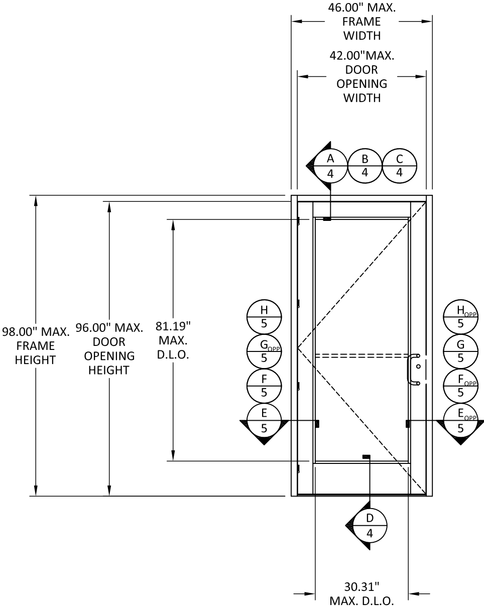
TYPICAL ELEVATION OUTSWING DOOR
