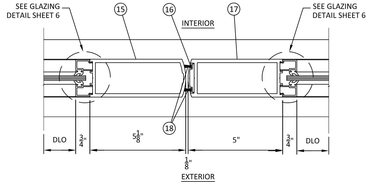
I 6 HORIZONTAL SECTION ASTRAGAL
