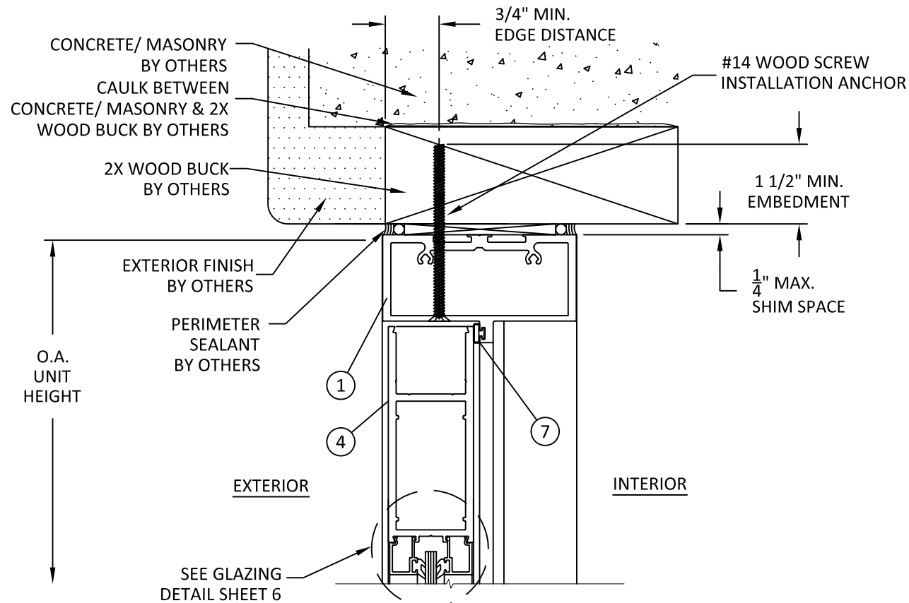
A 4 VERTICAL SECTION DOOR HEAD - 2X WOOD BUCK THROUGH FRAME
