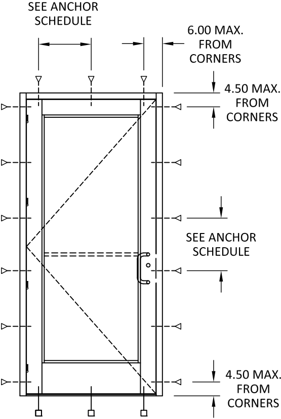
ANCHOR LAYOUT THROUGH FRAME OUTSWING DOOR
