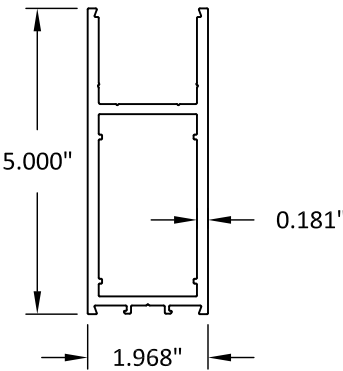
④ 5" TOP RAIL
