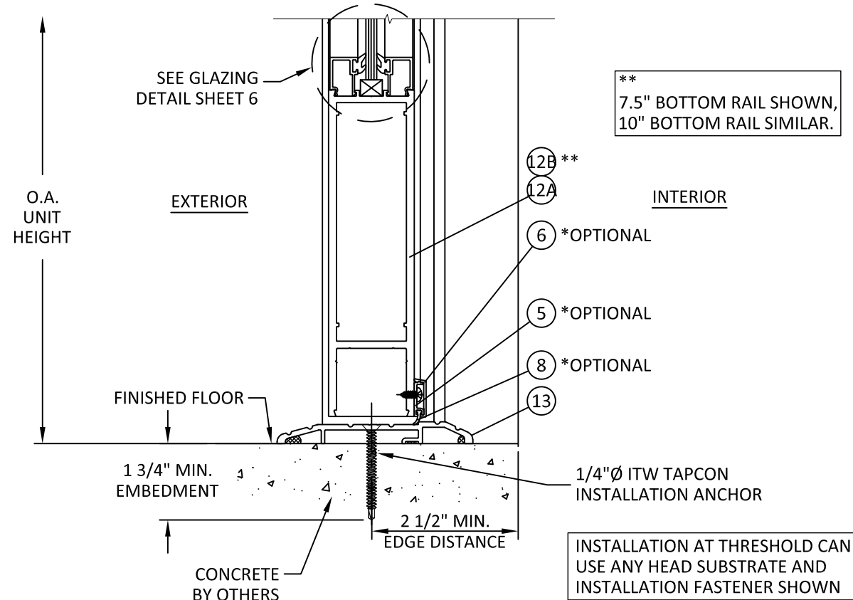
D 4 VERTICAL SECTION BOTTOM RAIL - CONCRETE
