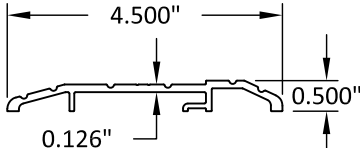
⑬ 4-1/2" DOOR THRESHOLD
